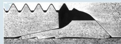
Cross section - Two-edge cutting ring
